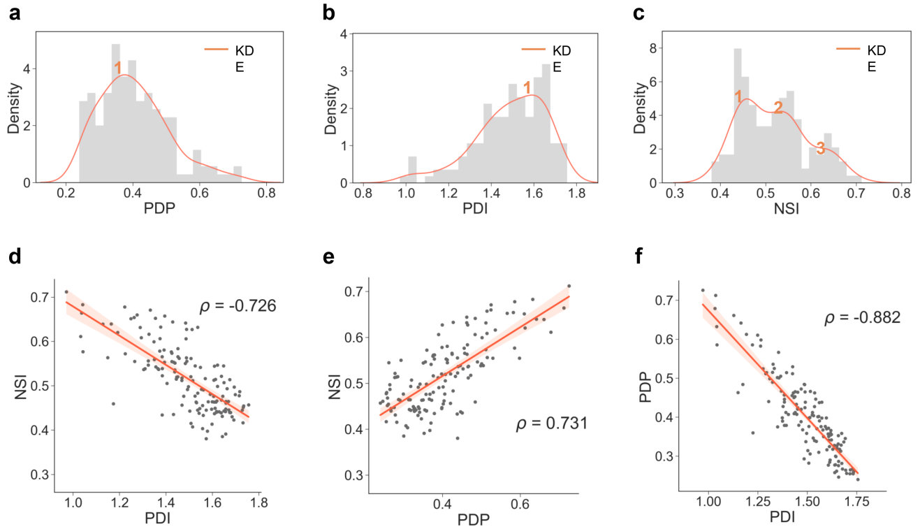
Supplementary Figure 7. Distribution of the pattern indicators and the pairwise correlations among them. a , b , and c are the histograms and kernel density estimate curves (KDEs), which describe the distribution of PDPs, PDIs and NSIs of cities of interest respectively. The numbers above the curves mark the peaks of the KDEs. d , e and f demonstrate the correlations between each pair of the three indicators, together with the corresponding Pearson correlation coefficient ( \rho ).
