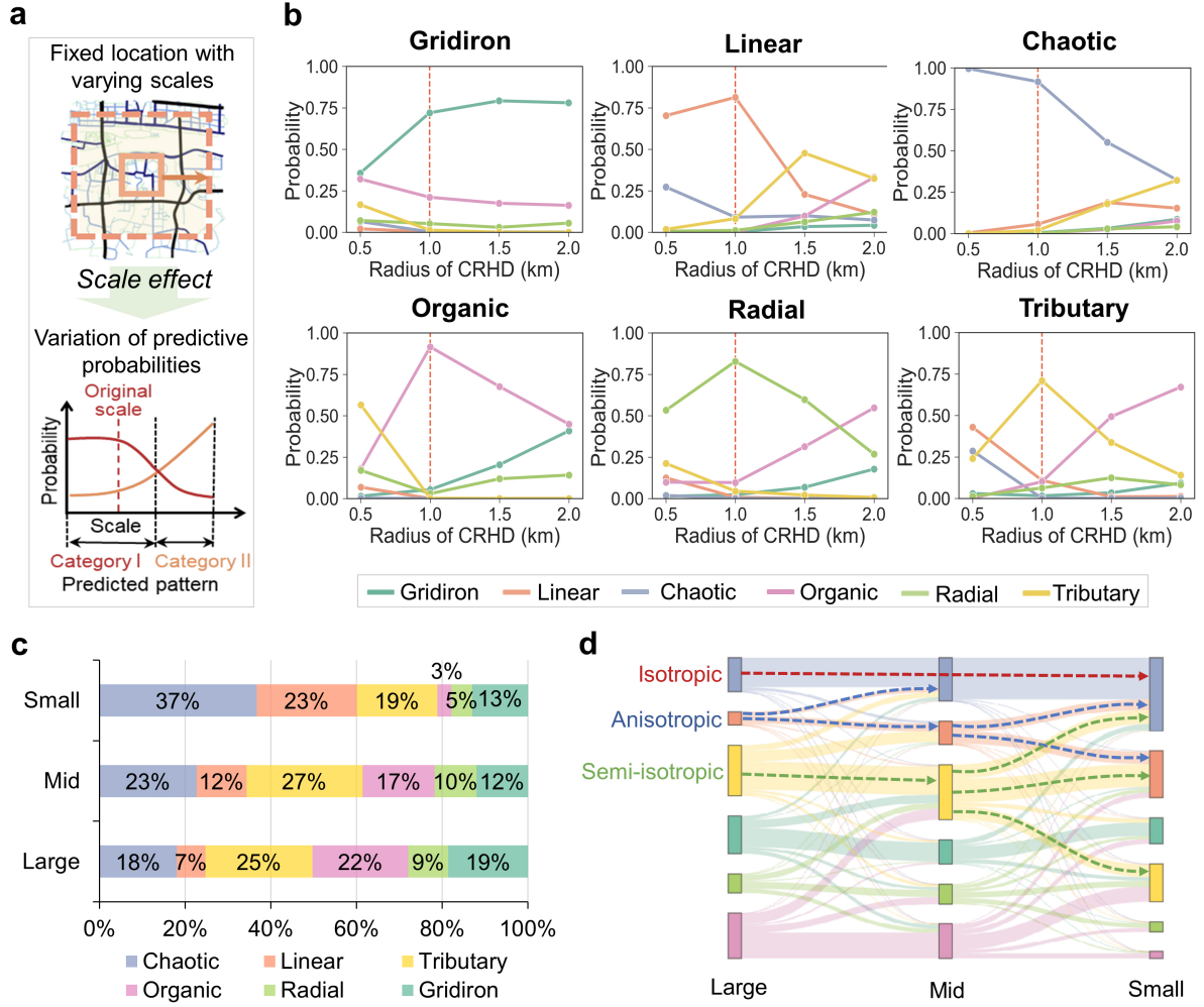
Figure 2: Scale effect on road network patterns. a The mechanism for evaluating the scale effect on road network patterns. b Scale-induced variations of predictive probabilities for each prior category. c Global pattern proportions at different scales. The global proportion of a pattern is the amount of grids pertaining to the pattern divided by the total amount of grids of all cities. d Global cross-scale mapping relations. There are two layers of mapping relations among the three scales, which are visualized by the Sankey diagram. The height of a node (i.e. pattern) denotes its proportion at the scale, while the width of a link indicates the proportion of aggregated cross-scale mapping relations from the larger scale to the smaller one (see detailed statistics in Supplementary Table 5).
