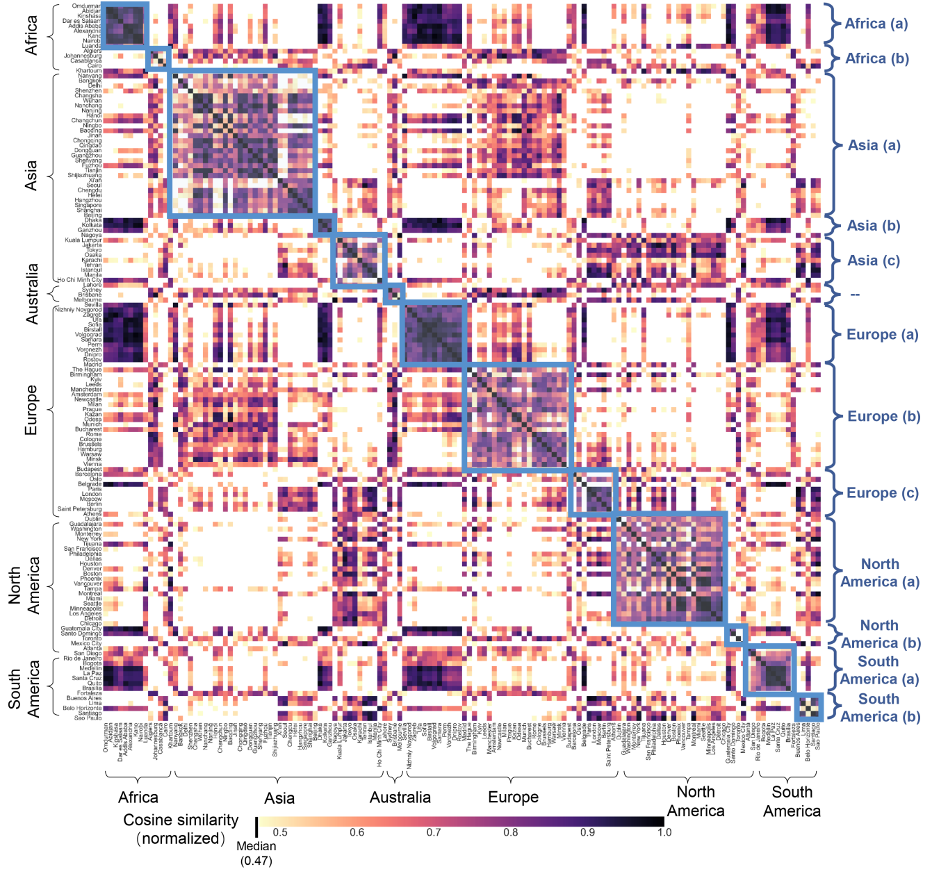
Supplementary Figure 6. Inter-city pattern similarity matrix. After pattern convolution, each city is embedded by the pattern proportions (a 18-dimension feature vector). The cities and their pattern proportions form a 144 \times 18 feature matrix. We standardize each column to be normally distributed, calculate the cosine similarity between each pair of cities, and obtain a 144 \times 144 similarity matrix. For easier interpretation, the cosine similarity scores are normalized to 0 to 1 by the maximum and minimum. Only the cells with the similarity score above the median (0.47) are visible. To discover the potential subgrouping among the cities, we reorder the similarity matrix in a special way. First, cities from the same continent are aligned together. Then, the cities in each continent are ranked by their average similarities with the cities in the same continent and those outside. Note that all the average similarities are replaced by ranges to loosen the constraint of absolute number size and inject more flexibility for grouping. The number of ranges are set as 4 with the best experimental performance. As we keep the similarity matrix symmetric, every square of dark cells on the diagonal indicates a potential subgroup of cities in the continent. There are totally 13 subgroups, including 2 in Africa, 3 in Asia, 1 in Australia, 3 for Europe, 2 for North America, and 2 for South America. The subgroups are annotated separately for each continent in alphabetical order.
