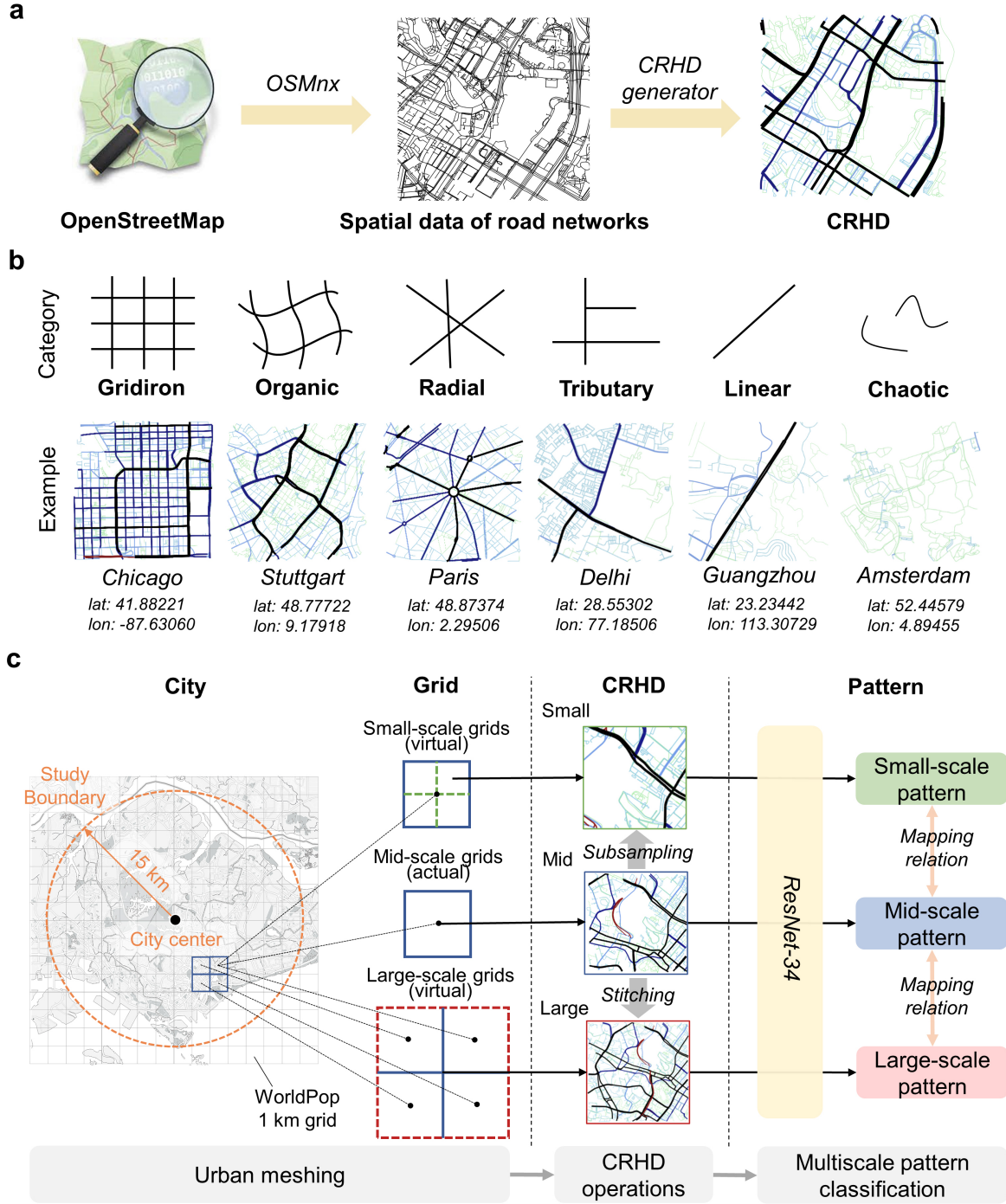
Figure 1: Workflow of urban meshing and multiscale road network pattern classification. a The workflow of generating a CRHD from OpenStreetMap (see details in Supplementary Note 1.1). b Our taxonomy of road network patterns with example CRHDs (1 km × 1 km). c The technical framework of multiscale road network pattern classification for a city (exemplified with Singapore), which consists of three major steps: urban meshing, CRHD operations, and multiscale pattern classification. Source of the raw street network data: (c) OpenStreetMap contributors.
