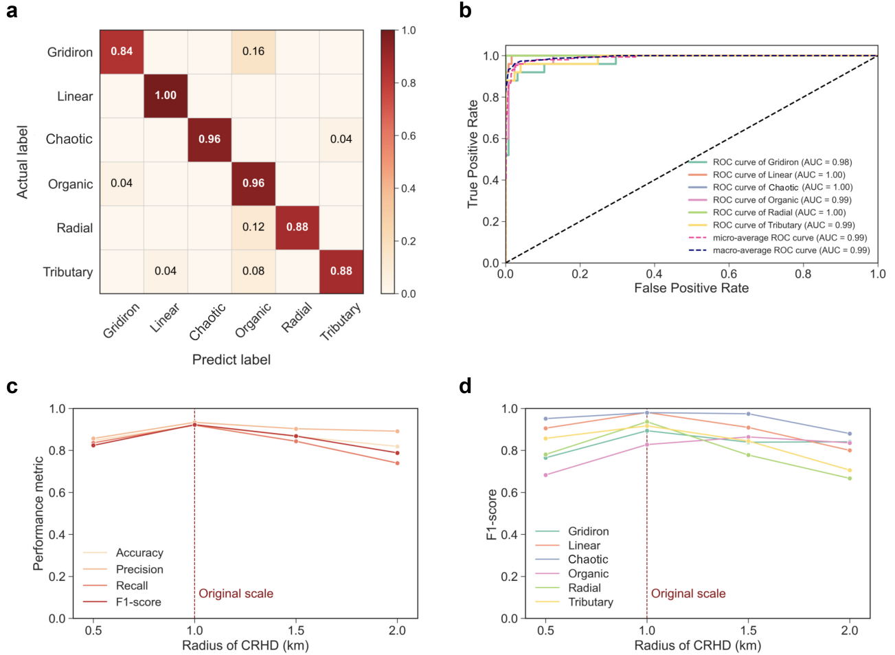
Supplementary Figure 2. Performance of the pattern classification model. a The confusion matrix evaluated by test set at original scale. The numbers on the diagonal denote the accuracy for each pattern. The numbers elsewhere refer to the rates of misclassifying the category in the row into the one in the column. b ROC curves and the corresponding AUC values of micro-average, macro-average and each category at original scale. c Variation of performance metrics (overall accuracy, precision, recall and f1-score) of the model at different scales. d Variation of f1-scores of individual categories at different scales.
