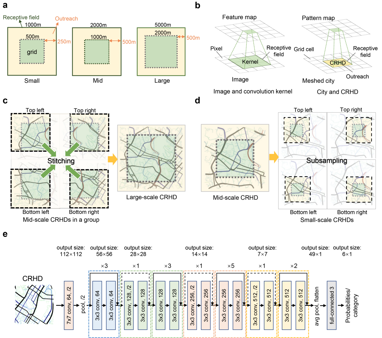
Supplementary Figure 1. Introduction of CRHDs, CRHD operations, and the architecture of the classification model. a The sizes of grids and corresponding CRHDs at small, mid, and large scales. The green squares in the middle are the urban grid and the yellow bounds represent the associated outreaches. Together, they constitute the receptive field of a CRHD. b The analogy between a convolution kernel and a CRHD. The process of classifying URN patterns by CRHDs is similar with conducting convolutions on images. The diagram shows the matchup of concepts between the two. c Stitching operation. It merges the CRHDs of four neighboring grids into a larger-scale one. The process is achieved by truncating the repetitive areas (edge areas) of the input diagrams and concatenating them based on pixel-level matching on the edges. After that, the width of outreaches remains the same. d Subsampling operation. It splits a CRHD into four smaller-scale ones that contain the road information of grids with outreaches in each corner. The operation is realized by slicing the CRHD by bounding boxes with varying positions. e The architecture of our pattern classification model (ResNet-34).
