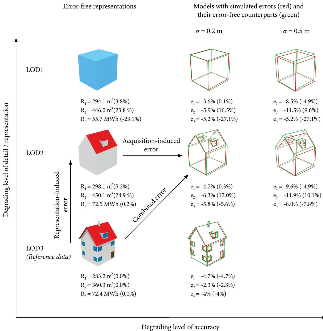
Figure 5. Illustration of a subset of the experiments and results of one simulation on a sample of one 3D building model disturbed according to two different levels of accuracy ( \sigma_{x,y,z} = 0.2 and 0.5 \text{ m} ). The results from the three considered spatial analyses are listed in the figure, and two types of errors are given for each case: the acquisition-induced error, and the combined error (in parentheses). This particular case is interesting because in the first two spatial analyses the LOD1 model inherently results in less inaccurate results than the LOD2 model.
