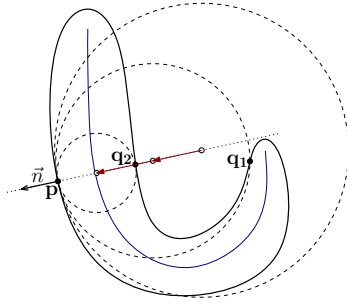
Figure 2: The shrinking ball algorithm.
